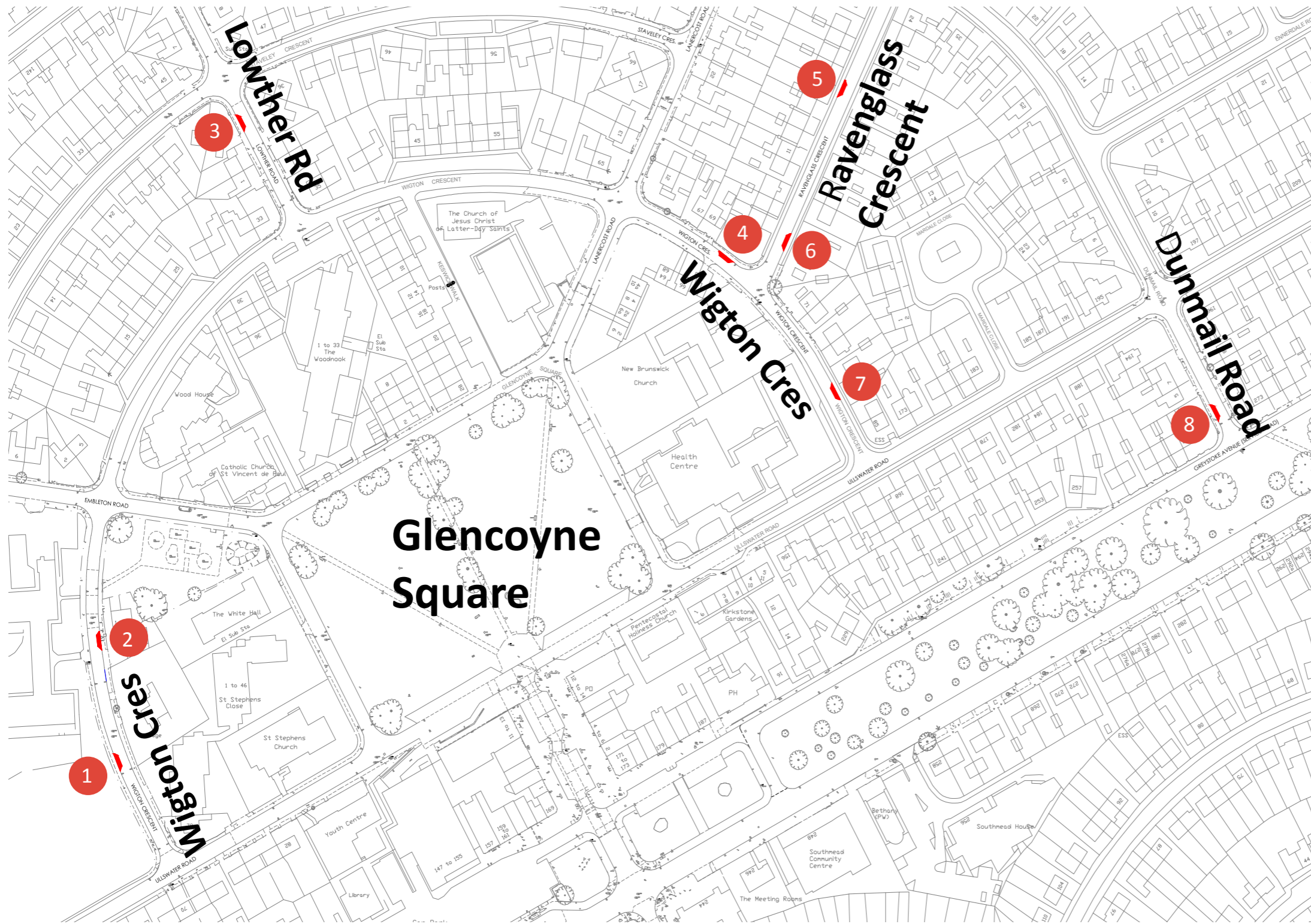
8 Proposed location of new SuDs pods
